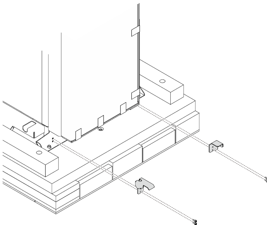
Figure 5. Retrait des supports
