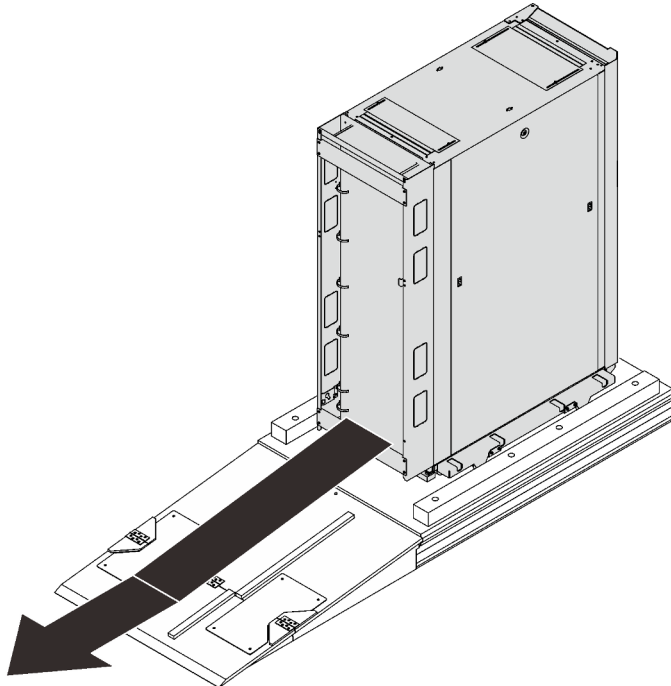
Figure 11. Moving the cabinet
