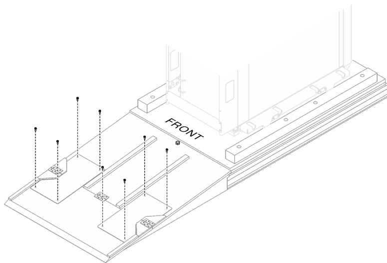
Figure 9. Securing the two plates to the ramp
