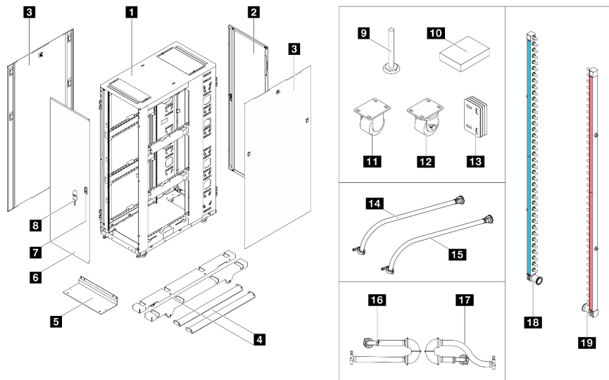
Figure 12. Parts listing
