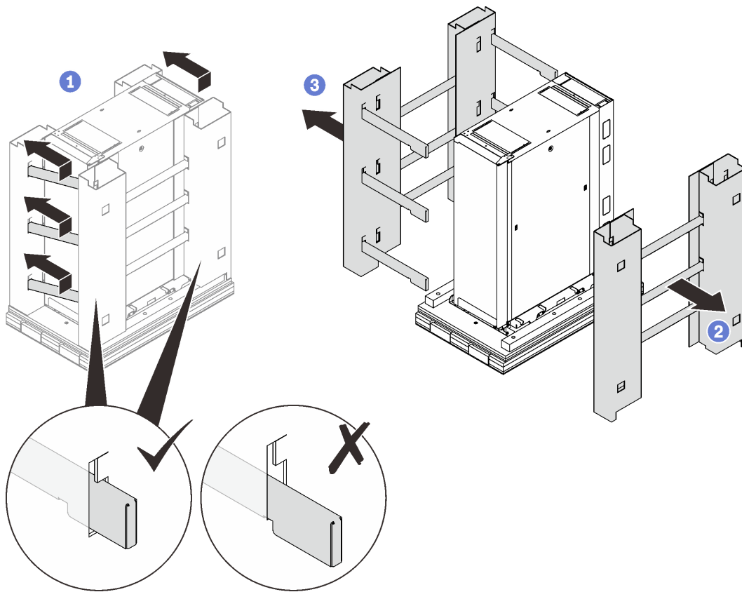
Figure 5. Removing the side frames
