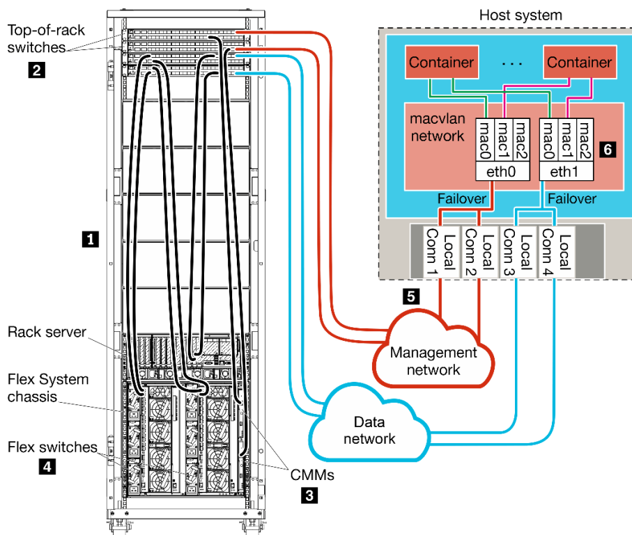
Figure 14. Sample physically separate data and management network topology for containers
