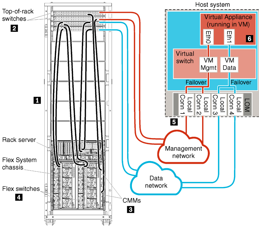
Figure 13. Sample physically separate data and management network topology for a virtual appliance
