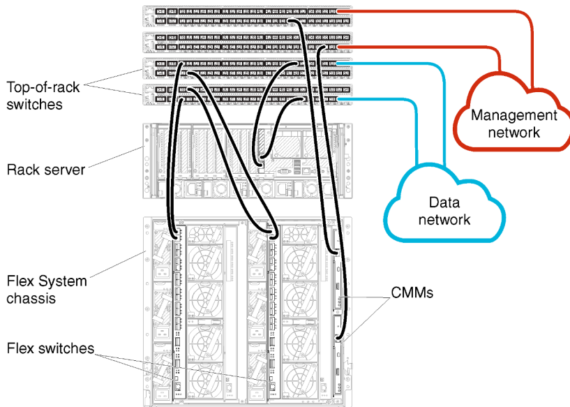
Figure 15. Example cabling for physically separate data and management networks
