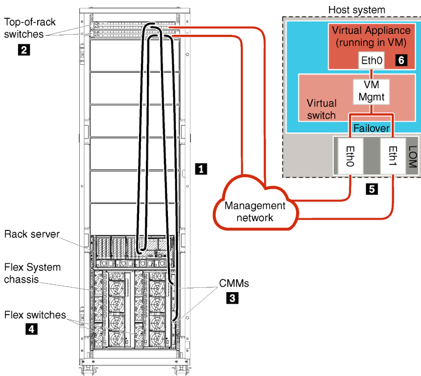
Figure 25. Sample management-only network topology for a virtual appliance
