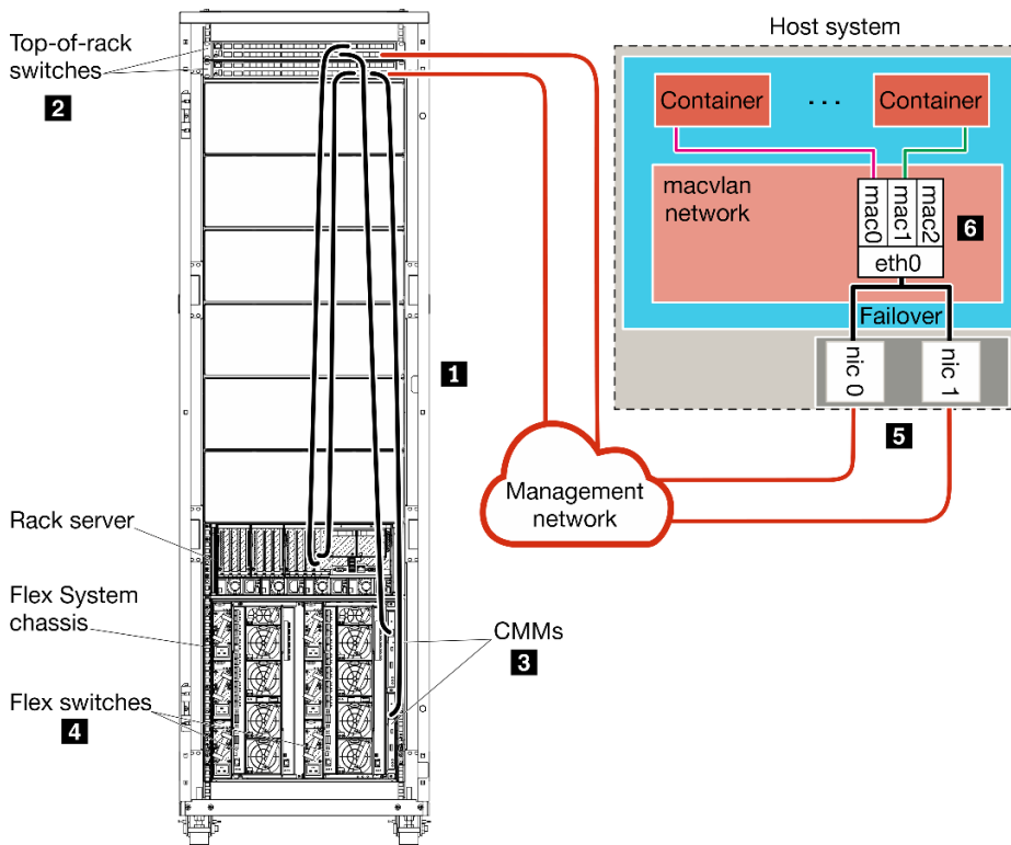
Figure 26. Sample management-only network topology for containers
