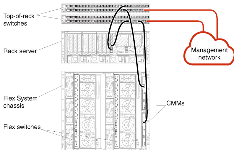
Figure 27. Example cabling for a management-only network
