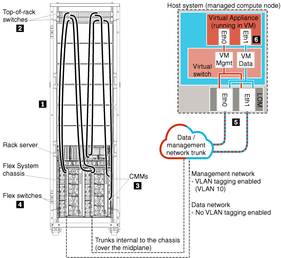
Figure 17. Sample virtually separate data and management network topology for a virtual appliance
