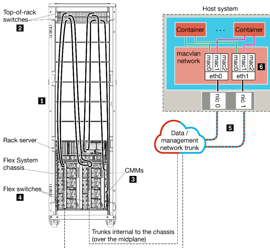
Figure 18. Sample virtually separate data and management network topology for containers
