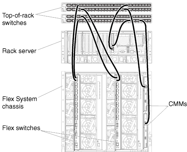
Figure 19. Example cabling for virtually separate data and management networks
