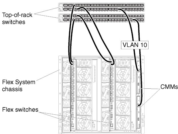
Figure 21. Example configuration for Flex switches on virtually separate data and management networks (VMware ESXi) in which VLAN tagging is enabled on the management network
