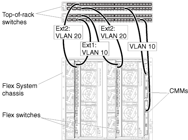
Figure 20. Example configuration for Flex switches on virtually separate data and management networks (VMware ESXi) in which VLAN tagging is enabled on both networks
