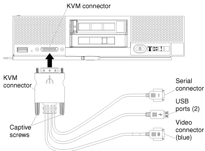
Figure 21. Console breakout-cable and front bezel of a server
