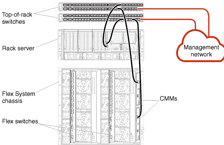
Figure 25. Example cabling for a management-only network
