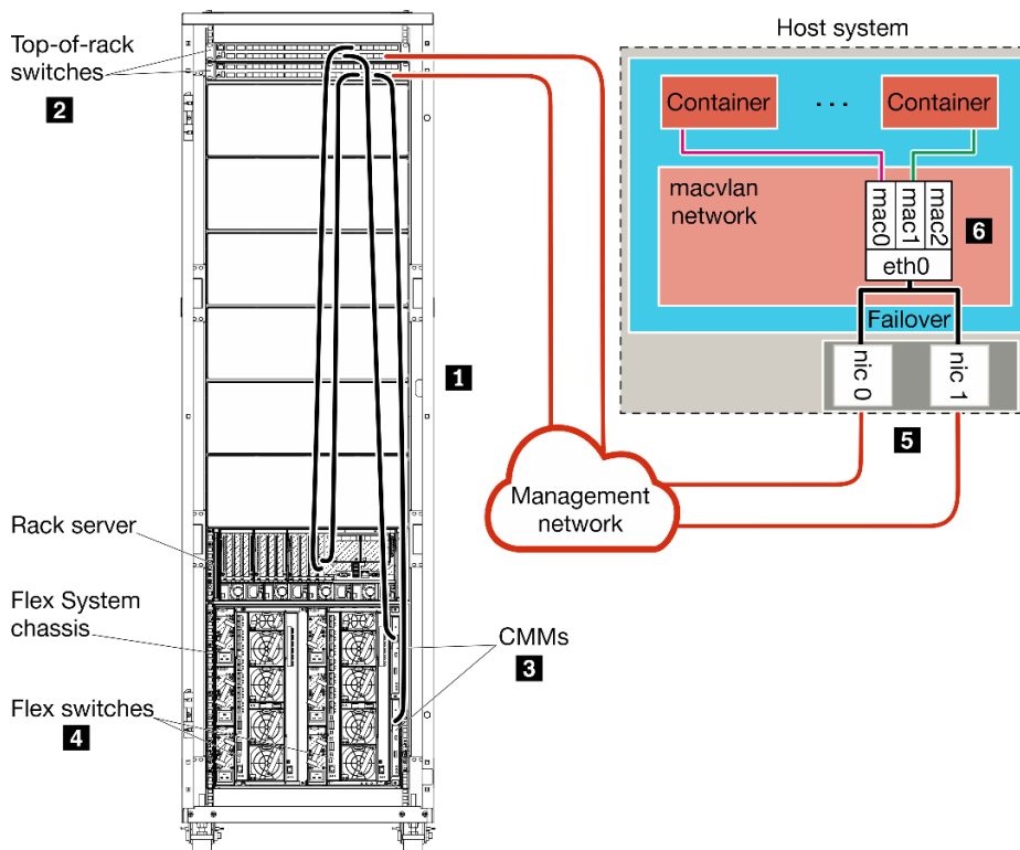
Figure 24. Sample management-only network topology for containers
