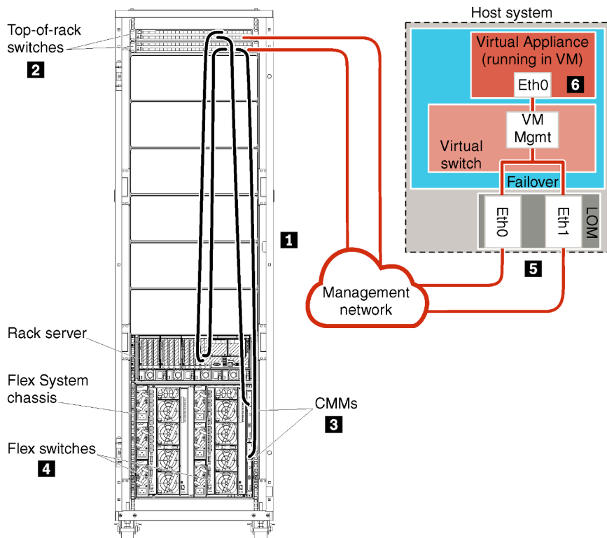
Figure 23. Sample management-only network topology for a virtual appliance
