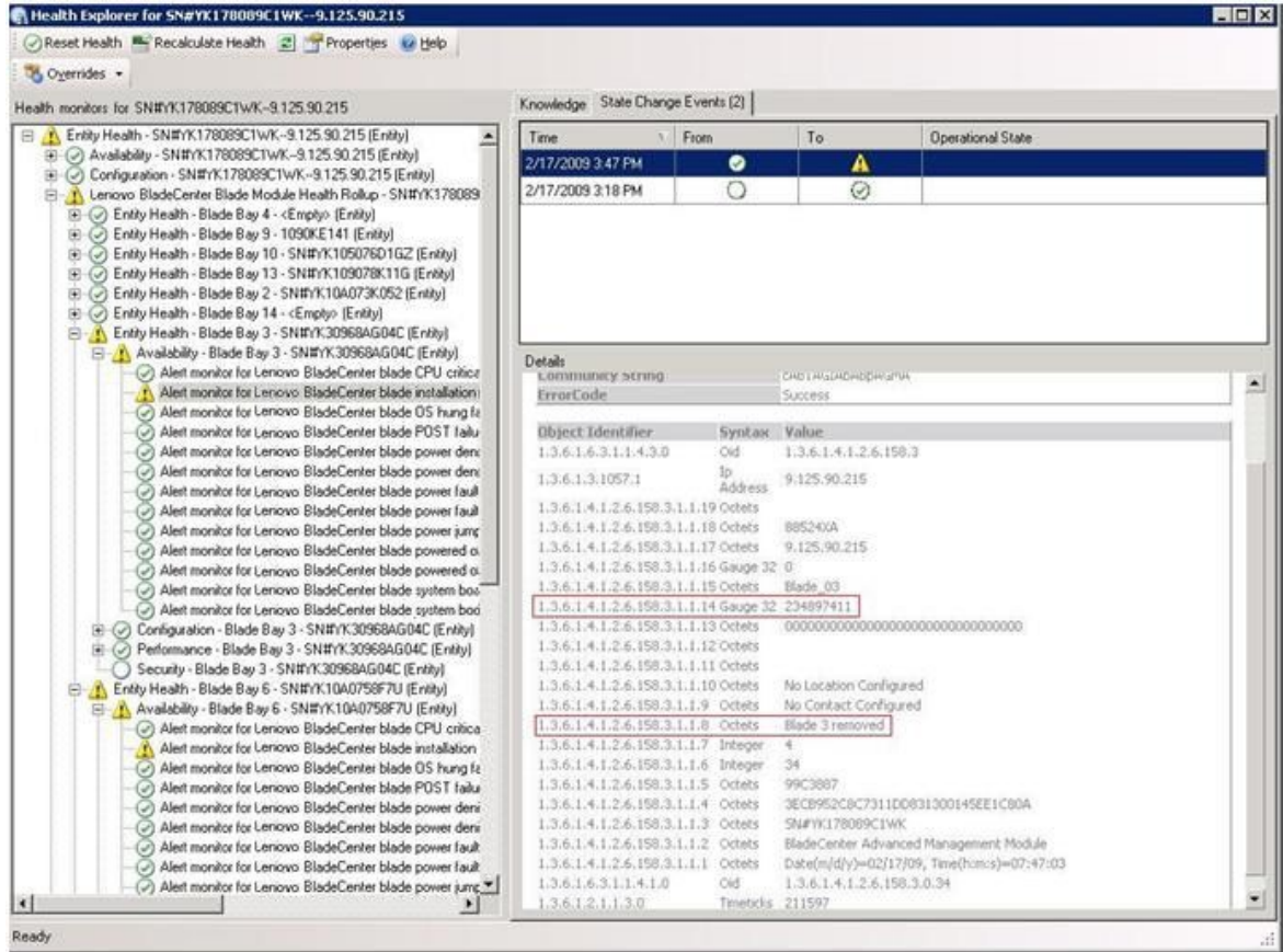
Figure 83. System x Windows Management Instrumentation (WMI) event
