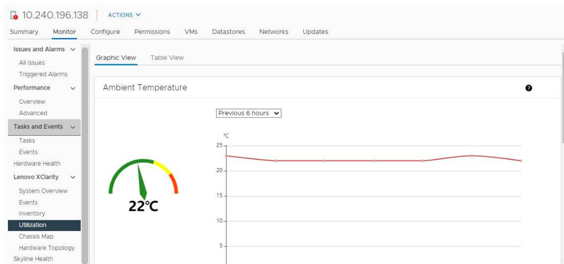
Figure 5. Utilization page
