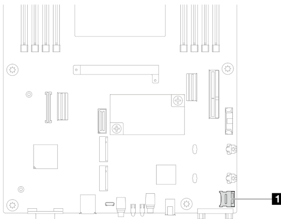
Figure 61. Emplacement du socket MicroSD
