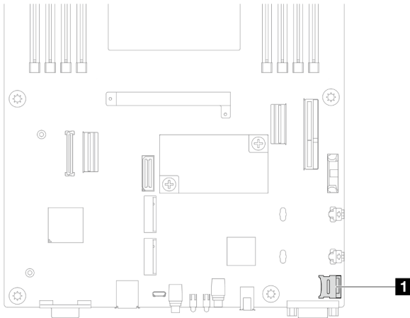
Figure 59. Emplacement du socket MicroSD
