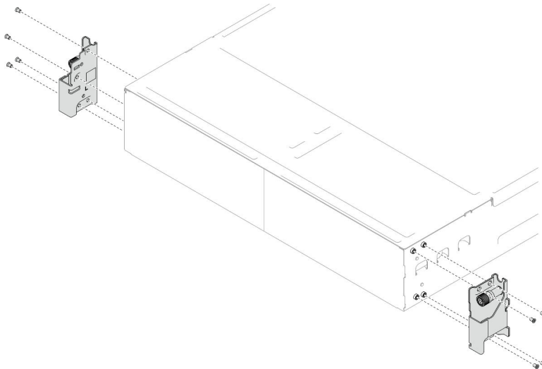
Figure 7. Installation des supports EIA
