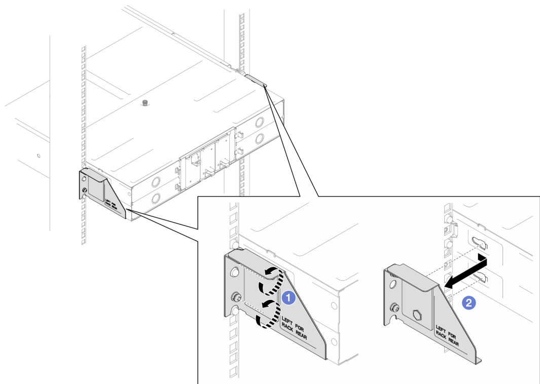
Figure 2. Retrait des supports de transport
