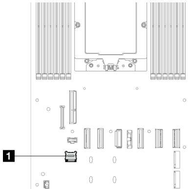
Figure 72. Emplacement du socket MicroSD
