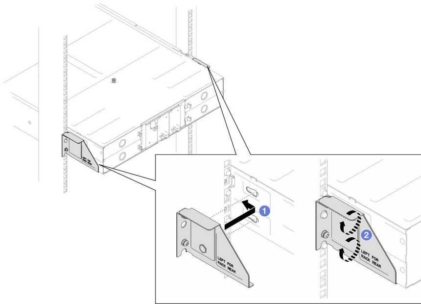
Figure 5. Installation des supports de transport
