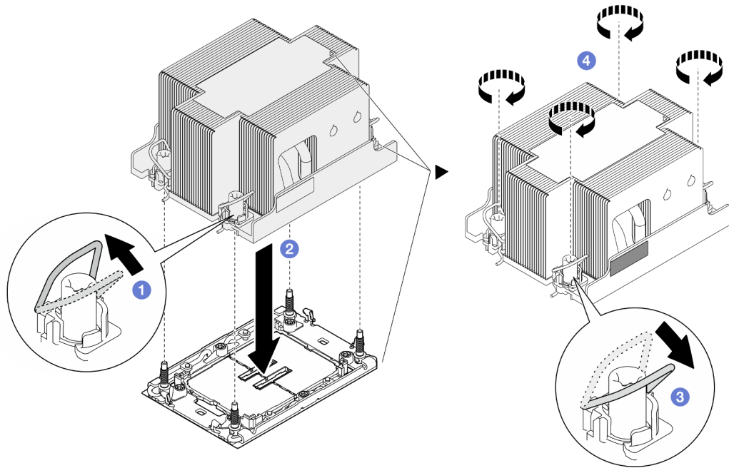
Figure 94. Installation d'un PHM standard 2U
