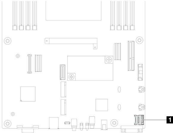
Figure 68. Emplacement du socket MicroSD
