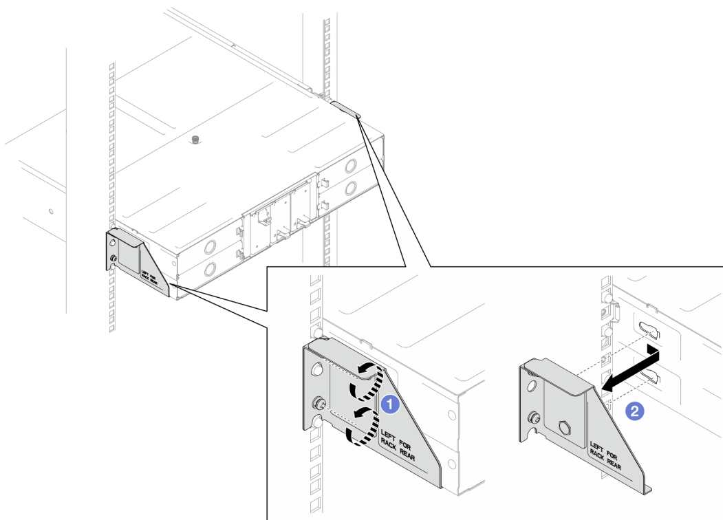
Figure 2. Retrait des supports de transport
