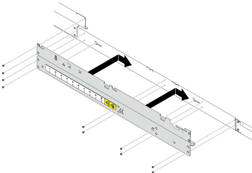
Figure 101. Installation du support latéral
