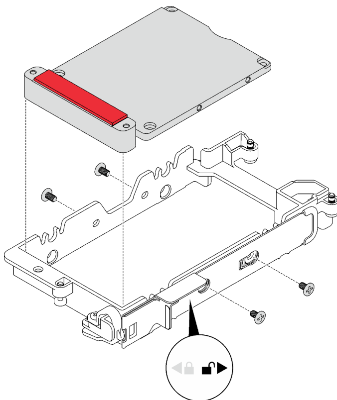
Figure 84. Retrait de la plaque de conduction
