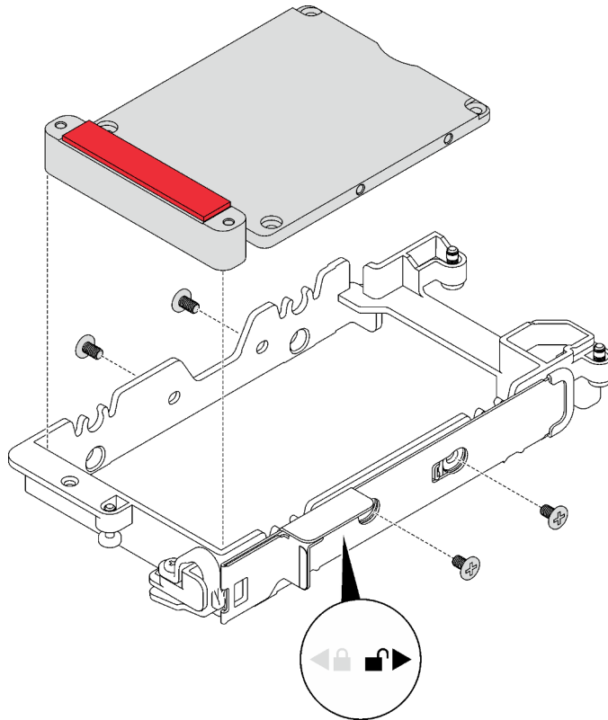
Figure 87. Installation d'une plaque de conduction
