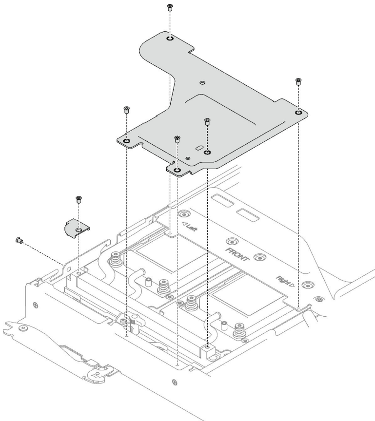
Figure 22. Retrait du support
