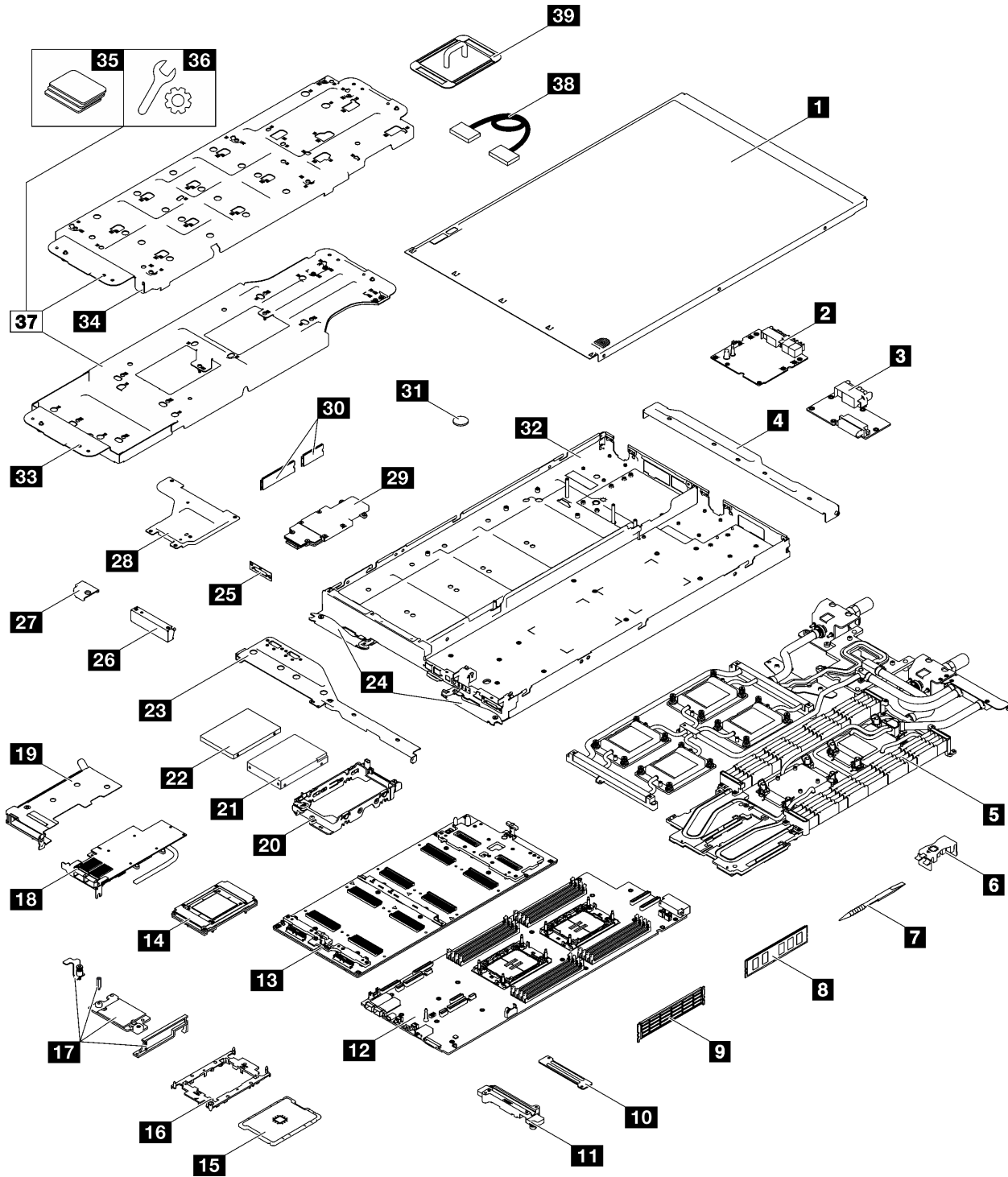
Figure 11. Composants SD650-I V3
