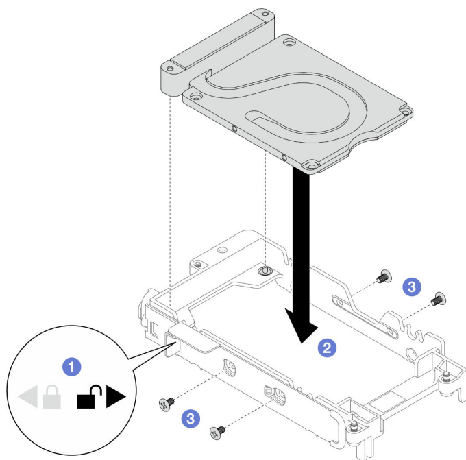
Figure 105. Installation d'une plaque de conduction
