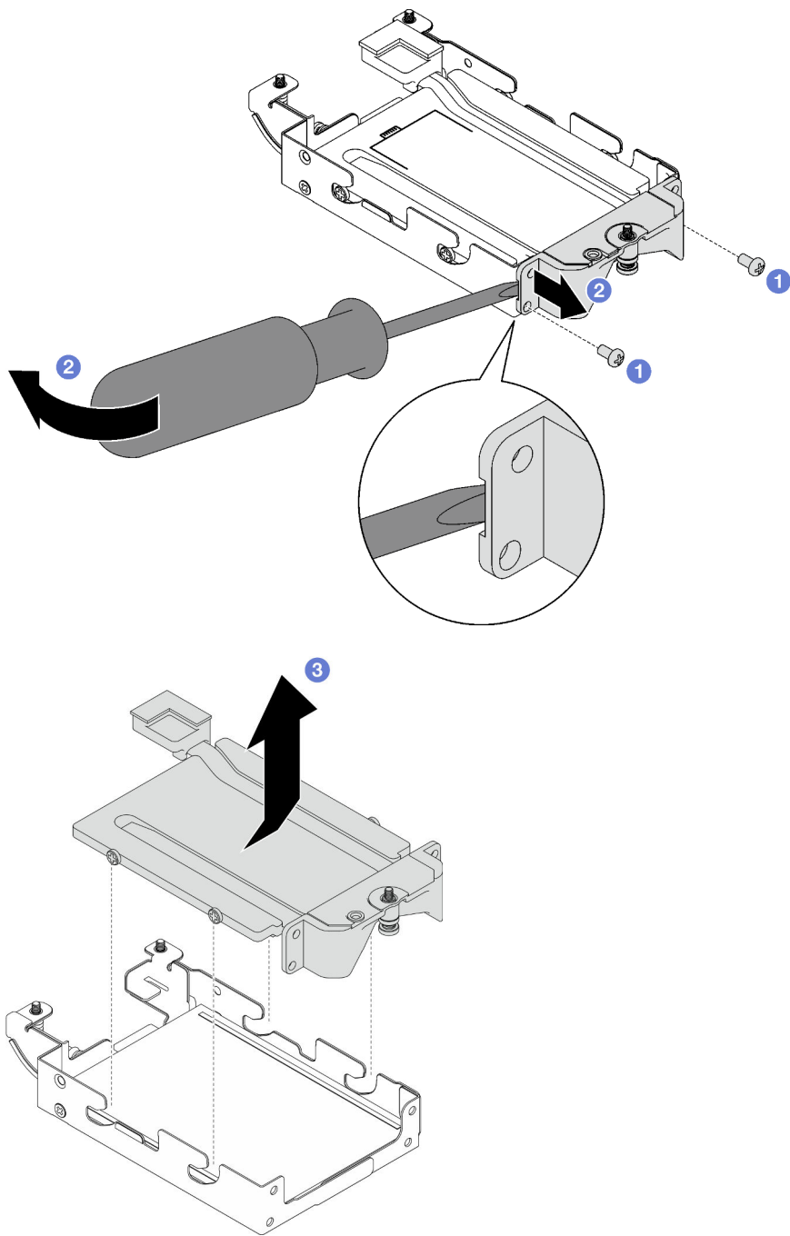
Figure 121. Retrait de la plaque de conduction
