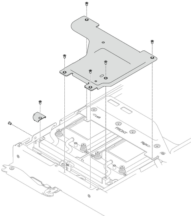
Figure 25. Installation du support
