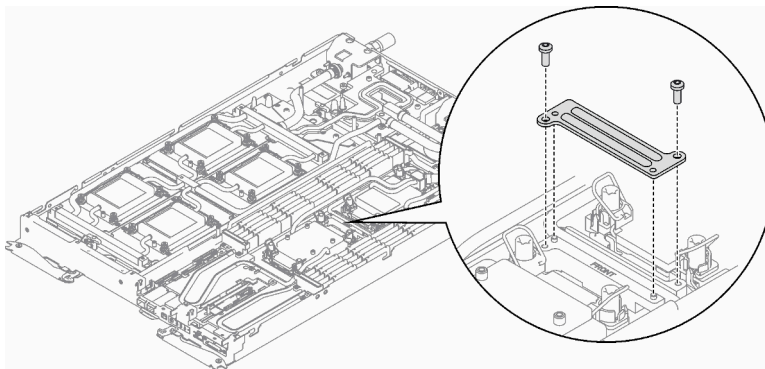
Figure 66. Installation de la plaque de serrage VR
