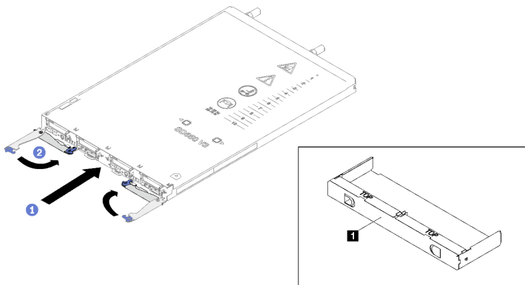
Figure 19. Installation du plateau
