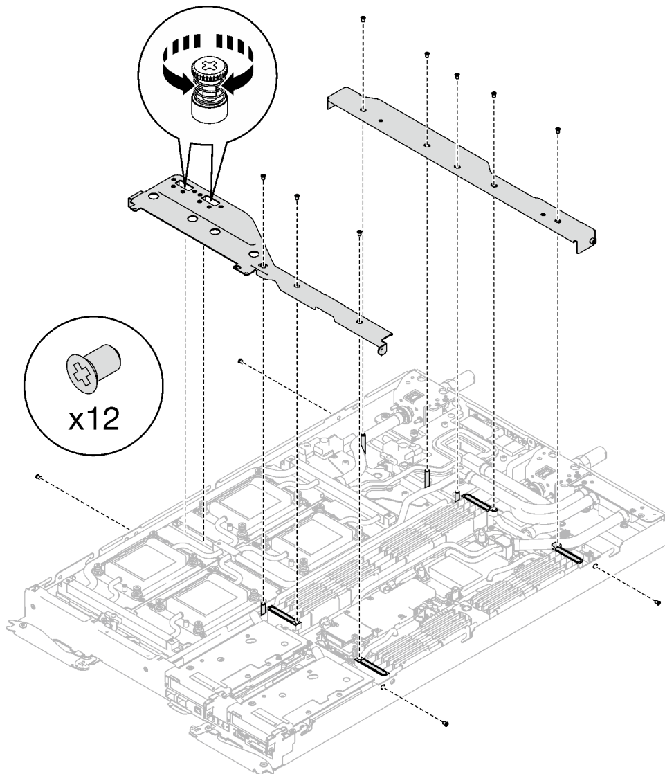
Figure 24. Installation des traverses (SD650-I V3)
