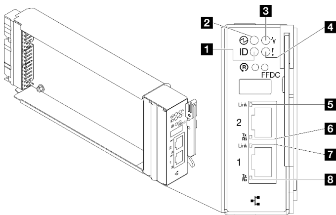
Figura 458. LED de SMM2
