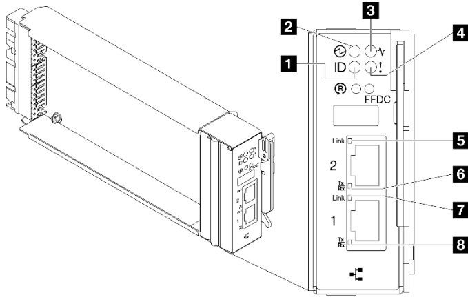
图 471. SMM2 LED
