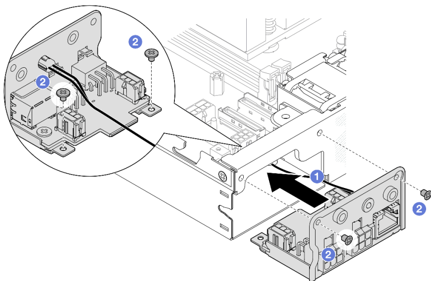
Figure 100. Installation du module DC PIB
