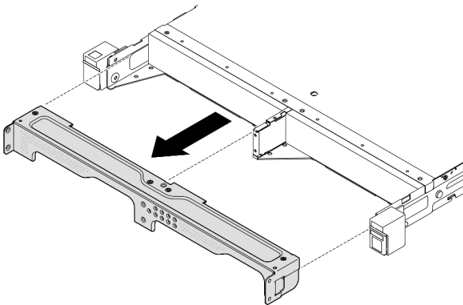
Figure 3. Retrait du support de transport
