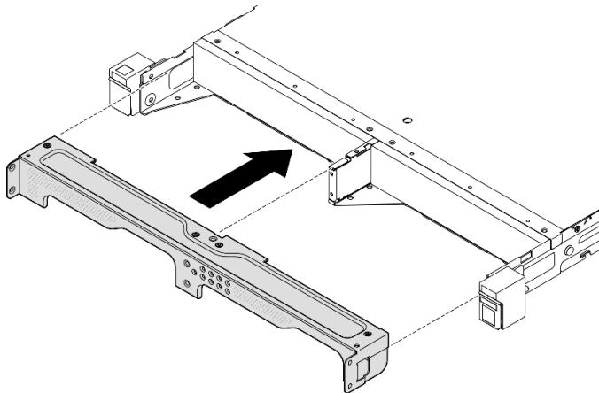
Figure 20. Installation d'un support de transport
