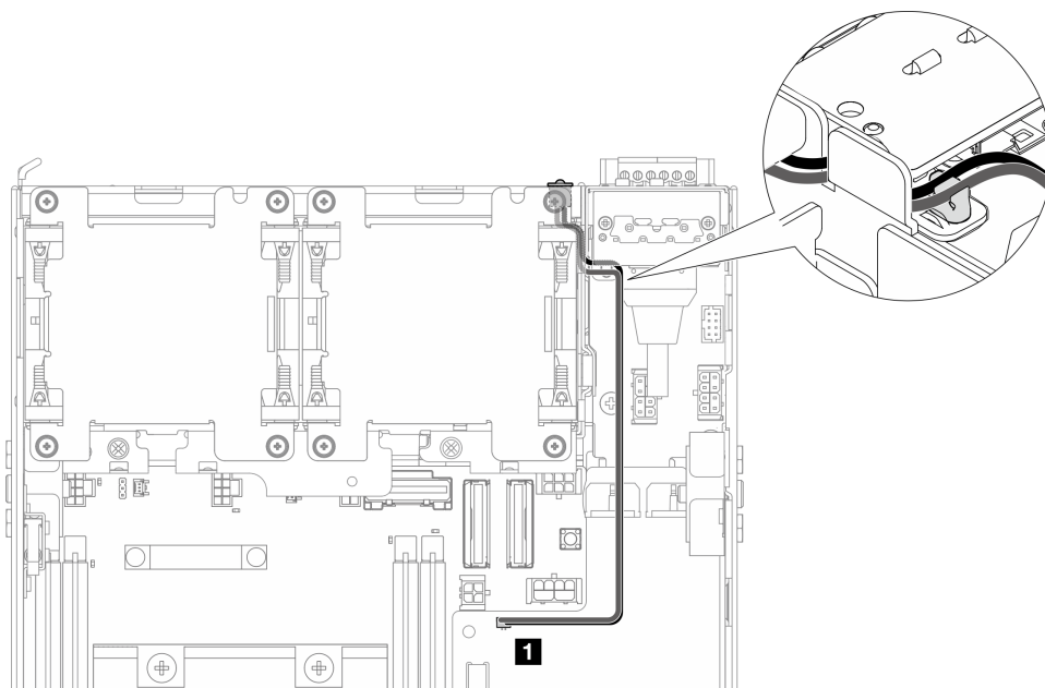
Figura 208. Cable de LED de PMB
