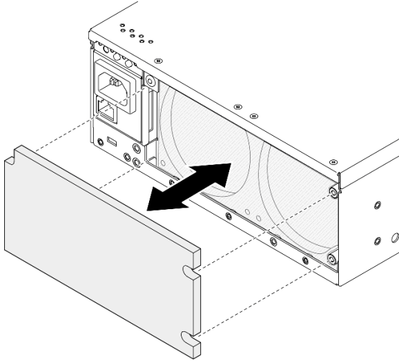
Figure 74. Installation du filtre anti-poussière
