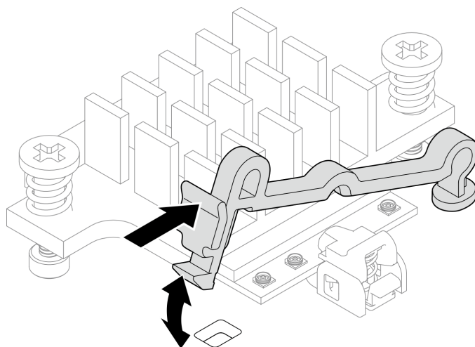
Figure 305. Insertion du support de câble
