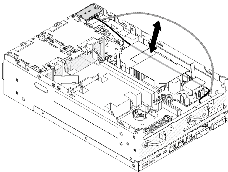
Figure 132. Placer le câble de signal
