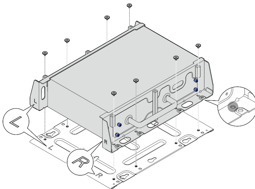
Figure 42. Installation de la plaque inférieure
