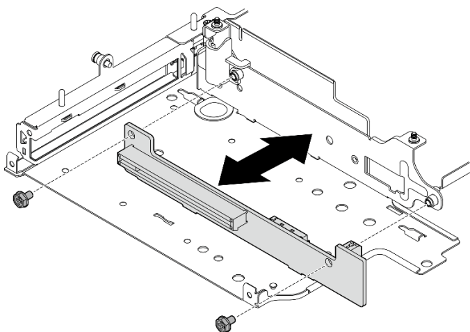
Figure 250. Installation de la carte mezzanine
