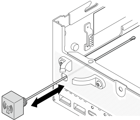
Figure 103. Installation de l'antenne Bluetooth
