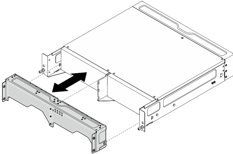
Figure 3. Retrait du support de transport
