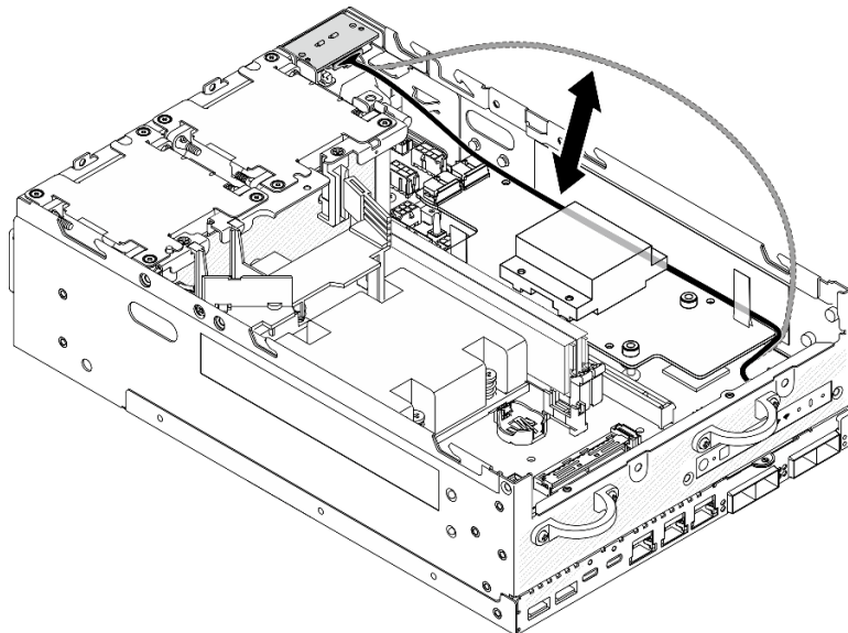
Figure 207. Placer le câble de signal
