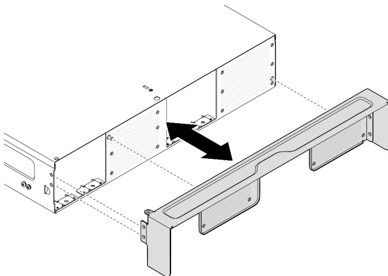
Figure 12. Installation du support de transport
