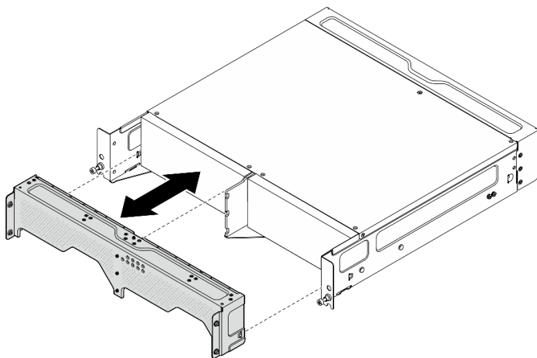
Figure 70. Installation du support de transport
