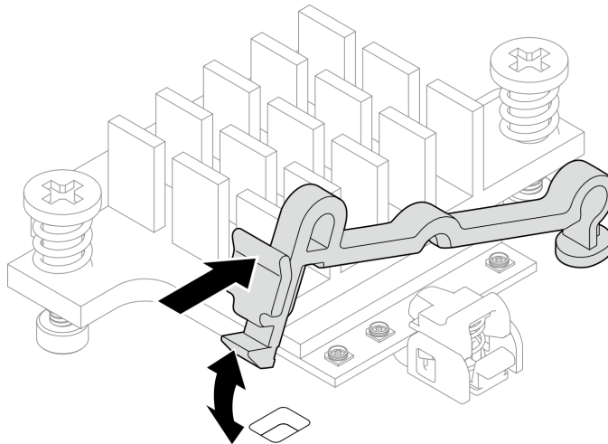
Figure 312. Soulever le support de câble
