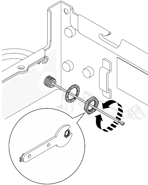
Figure 104. Installation de l'antenne Bluetooth
