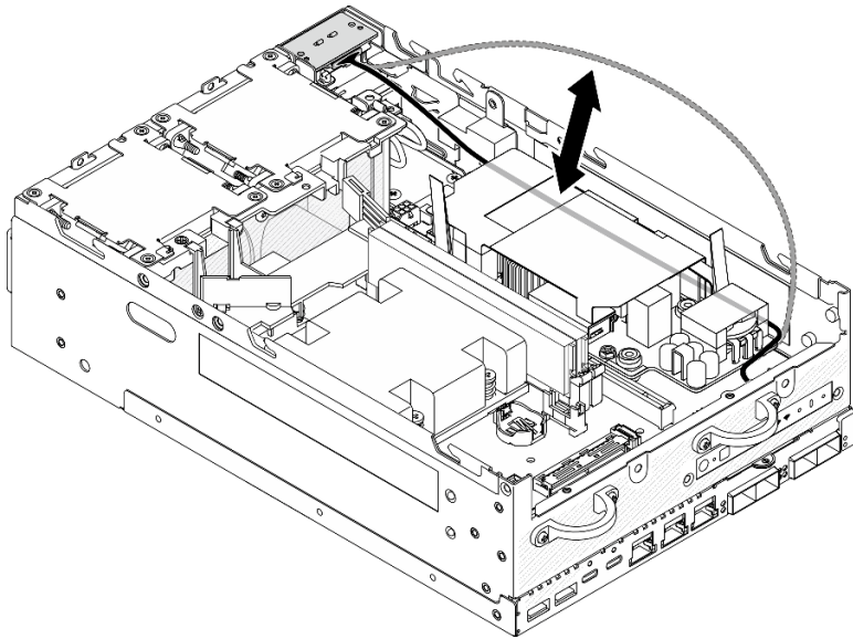
Figure 137. Placer le câble de signal
