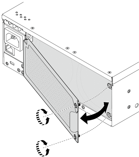
Figure 75. Installation du panneau
