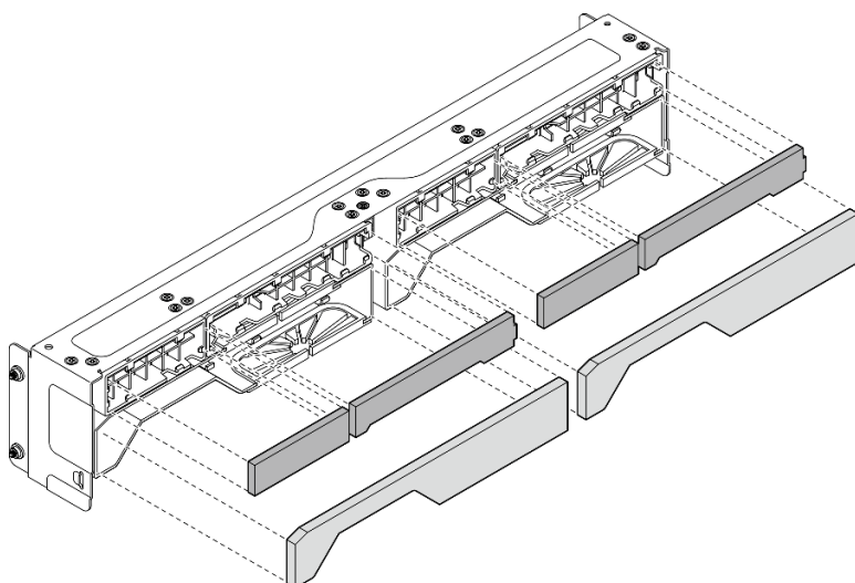
Figure 69. Installation des filtres anti-poussière
