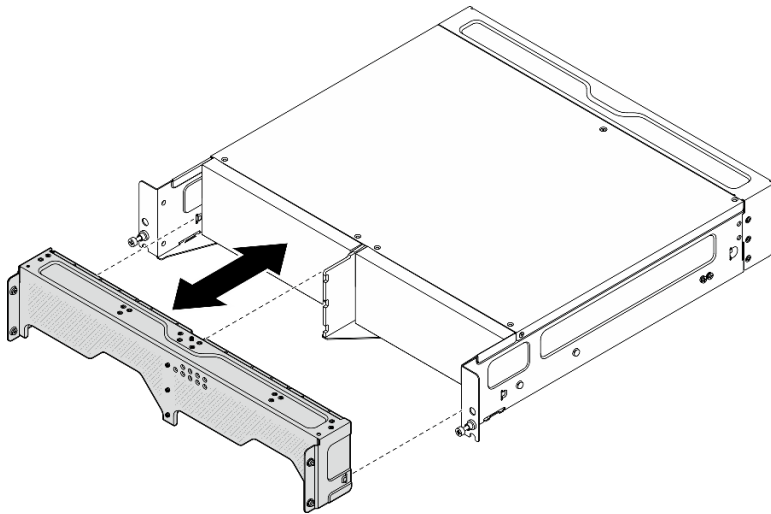
Figure 24. Installation du support de transport
