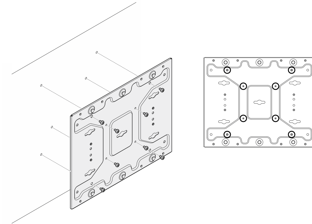
Figure 44. Installation de la plaque de montage mural
