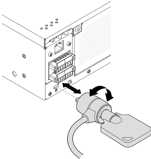
Figure 164. Installation du verrou Kensington
