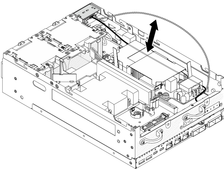
Figure 141. Placer le câble de signal
