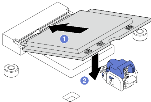
Figure 287. Installation du module WLAN/Bluetooth
