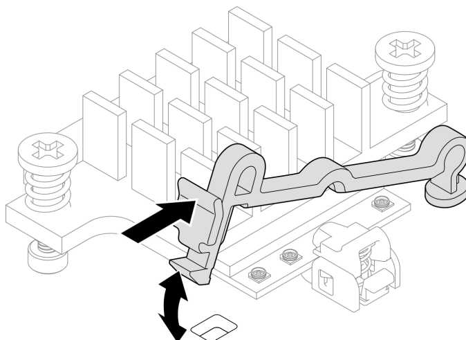
Figure 316. Insertion du support de câble
