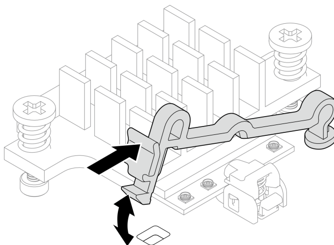
Figure 293. Insertion du support de câble
