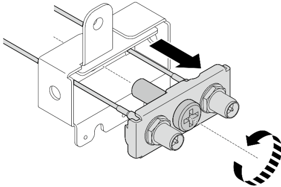
Figure 318. Retrait du support
