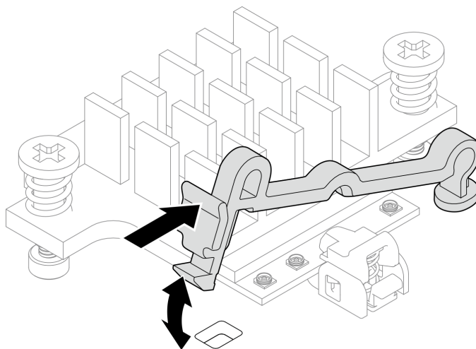
Figure 109. Insertion du support de câble
