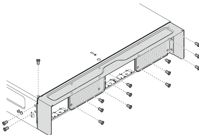
Figure 13. Serrer les vis
