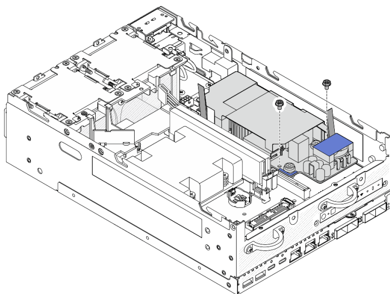
Figure 139. Serrer les vis
