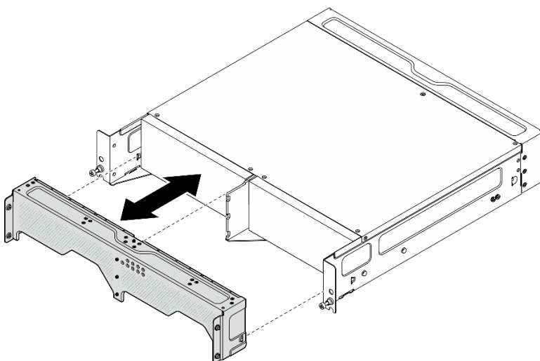
Figure 67. Retrait du support de transport
