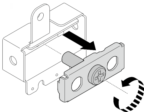
Figure 324. Retrait du support
