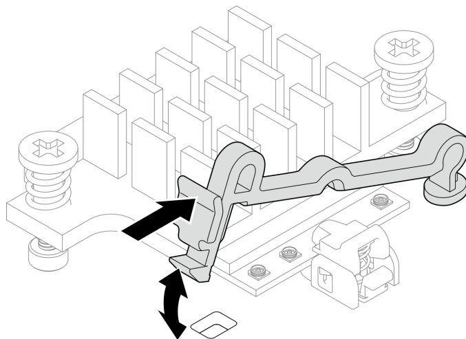
Figure 301. Soulever le support de câble
