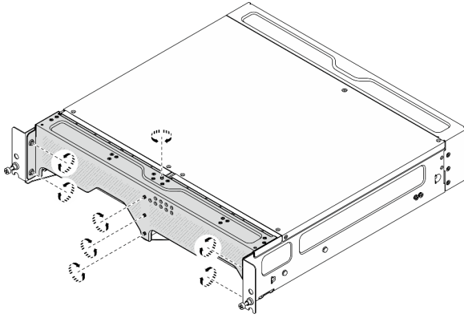
Figure 71. Serrer les vis
