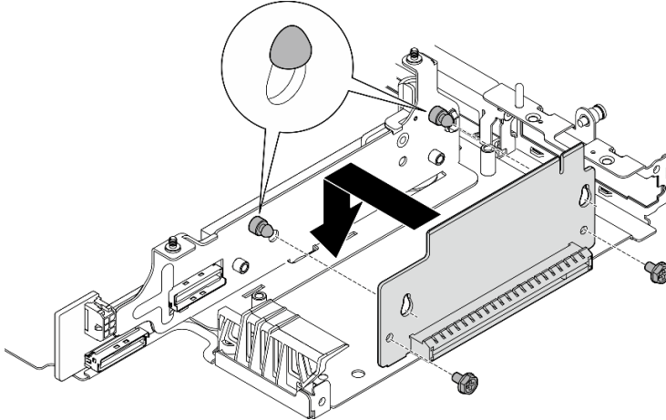
Figure 244. Installation de la carte mezzanine
