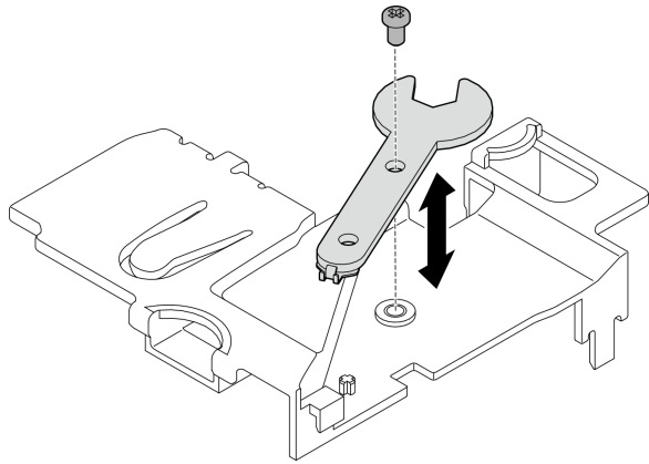
圖例 102. 鬆開扳手
