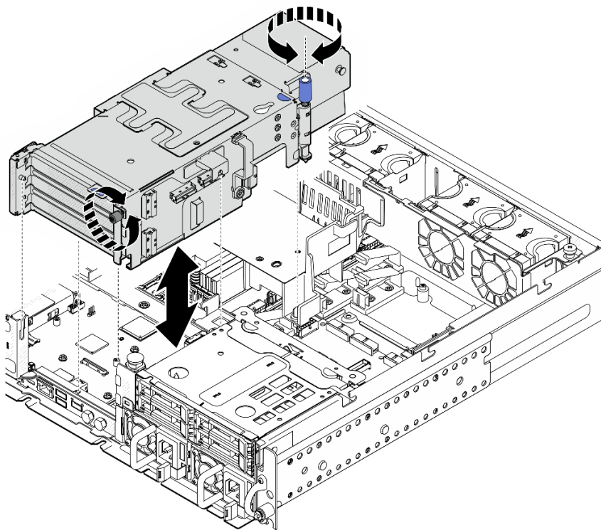
Figure 137. Installation du bloc mezzanine PCIe 2
