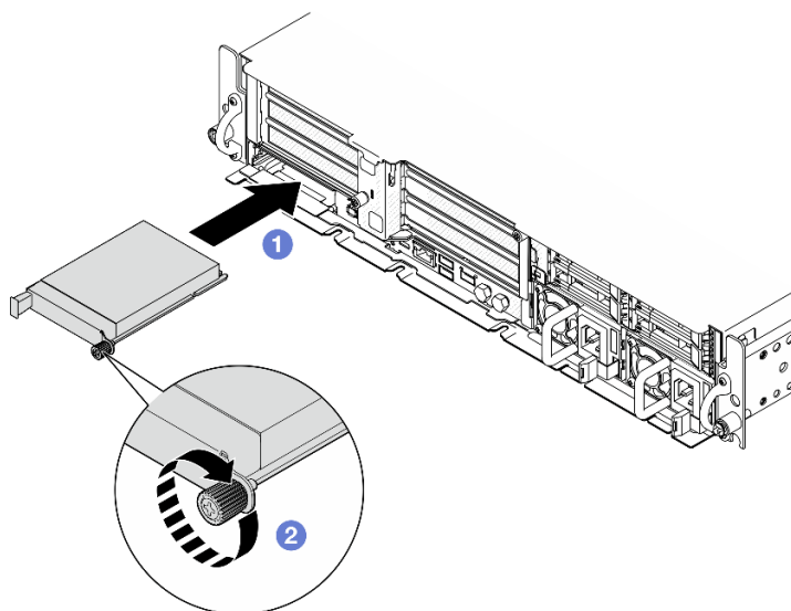
Figure 105. Installation du module OCP
