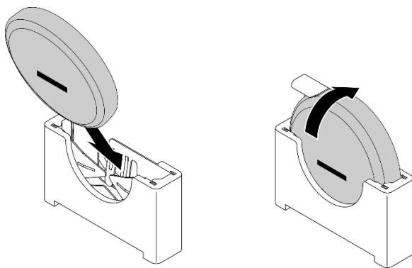
Figure 47. Installer la pile CMOS
