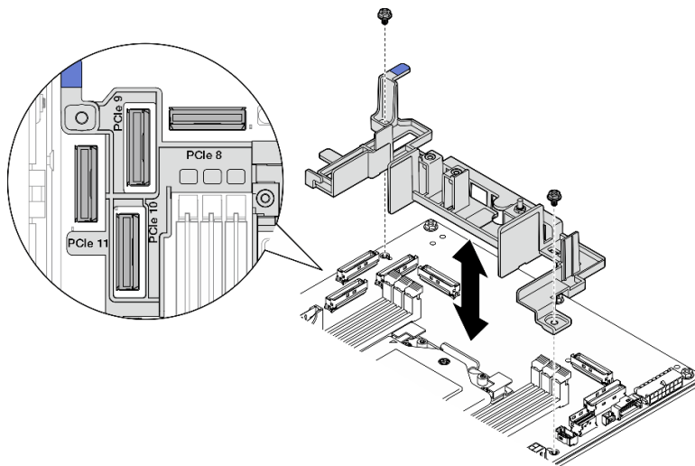
Figure 43. Installation du support de câbles
