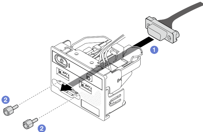
Figure 117. Installation du câble VGA
