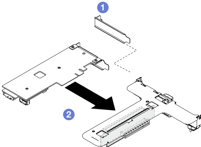
Figure 70. Installation de l'adaptateur PCIe (emplacement 2)
