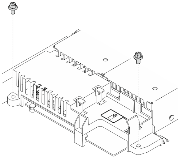
Figure 93. Installation des vis du carter PDB
