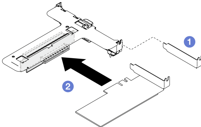
Figure 69. Installation de l'adaptateur PCIe (emplacement 1)
