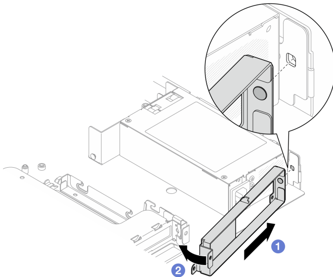
Figure 79. Installation du support arrière
