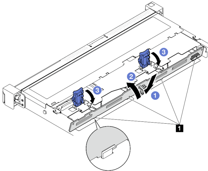
Figure 13. Installation de la plaque arrière
