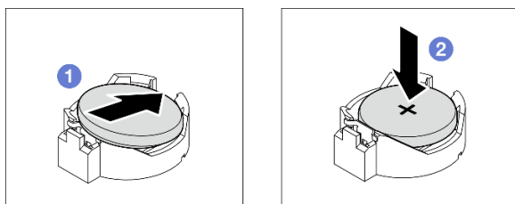
Figure 23. Installation de la pile CMOS
