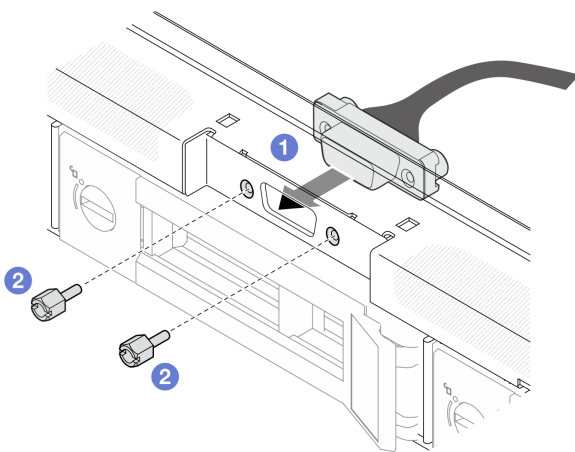
Figure 120. Installation du câble VGA
