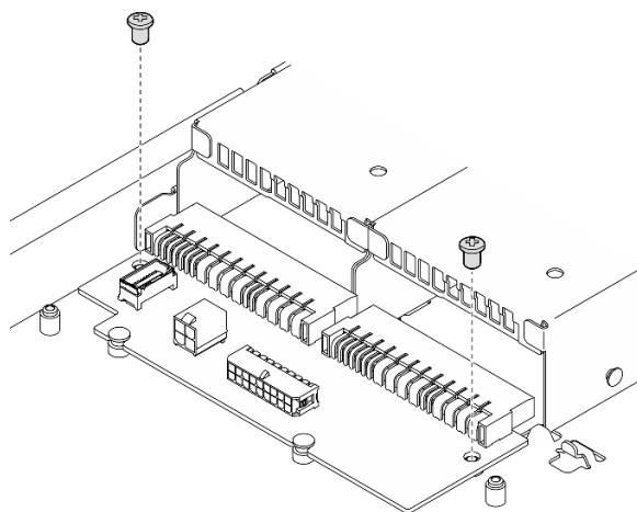
Figure 91. Installation des vis
