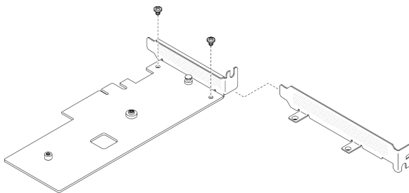
Figure 55. Installation d'un support extra-plat
