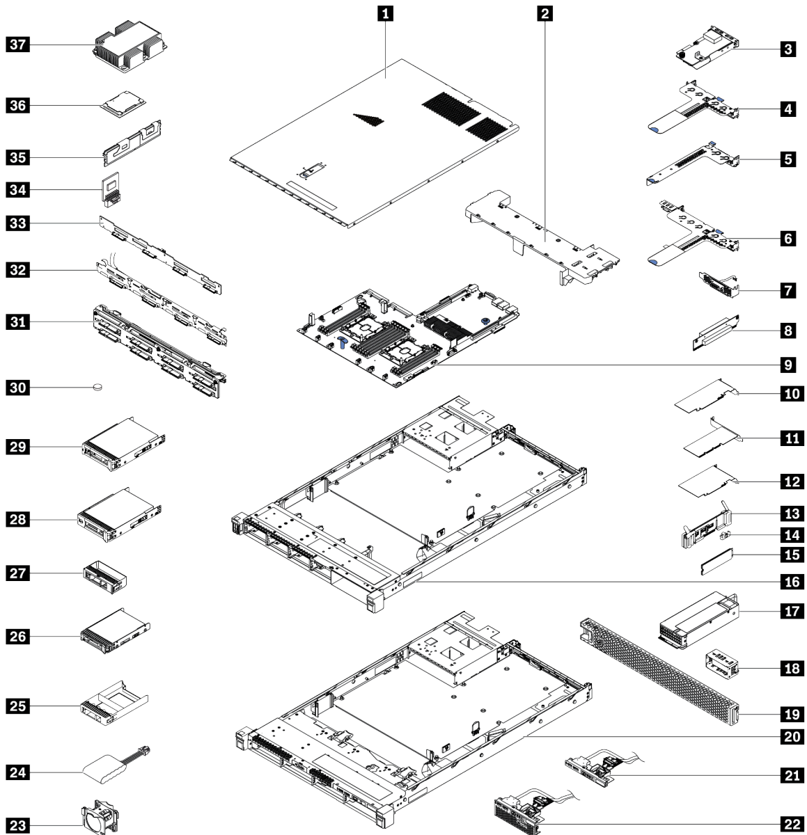
Figure 18. Composants serveur
