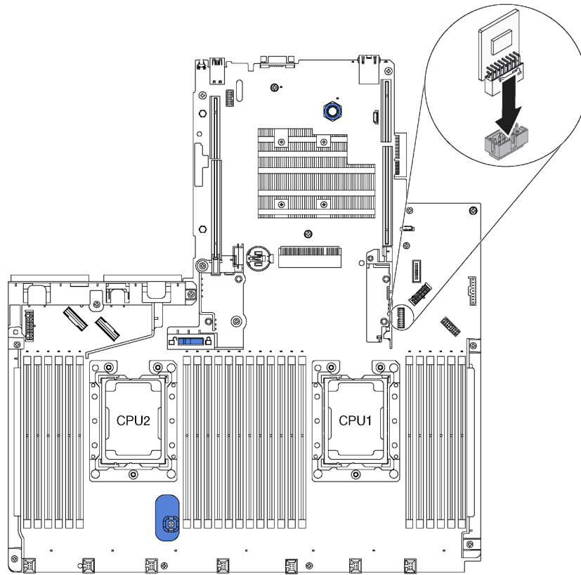
Figure 103. Installation d'adaptateur TCM/TPM
