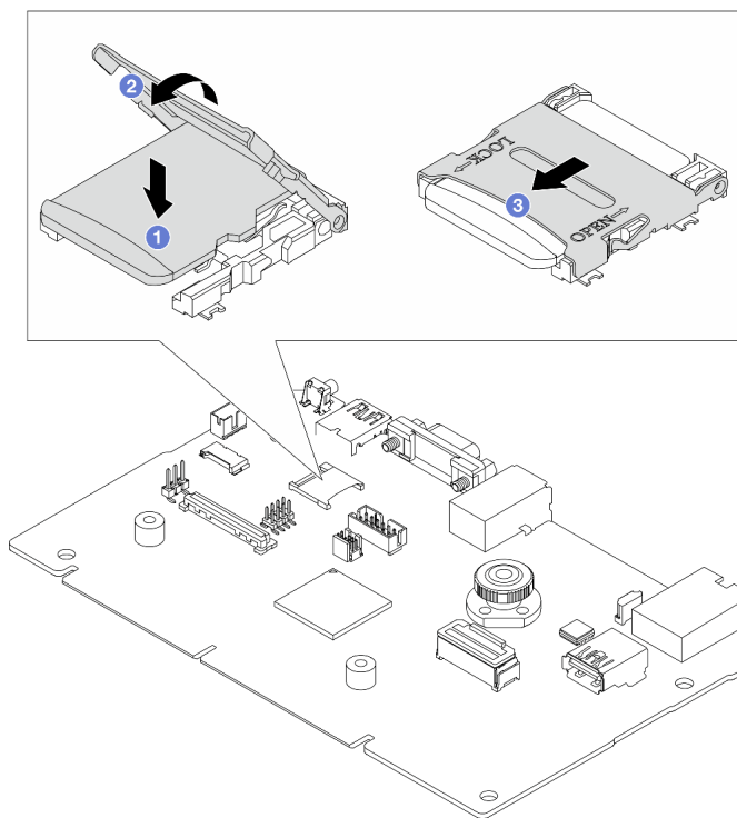
Figure 86. Installation de la carte microSD
