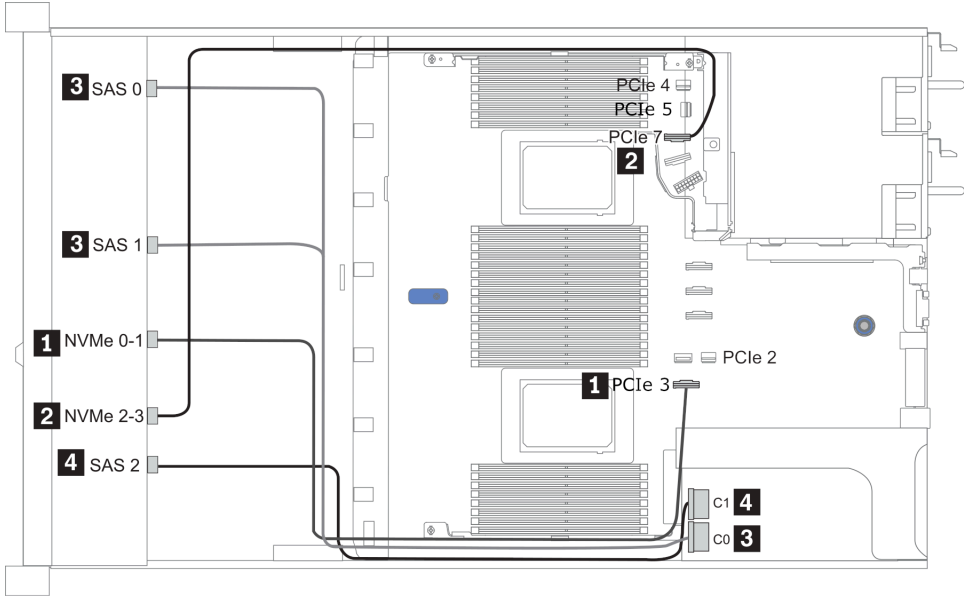
圖例 26. Configuration 2 (2 CPU installed)
