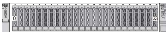
Figure 5. Front view with 24 x 2.5-inch drive bays
