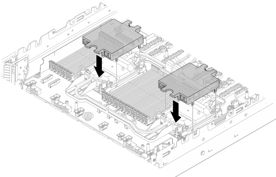
Figura 99. Instalando as tampas de placa fria
