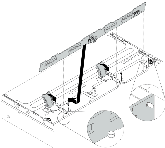
Figura 105. Instalando o backplane
