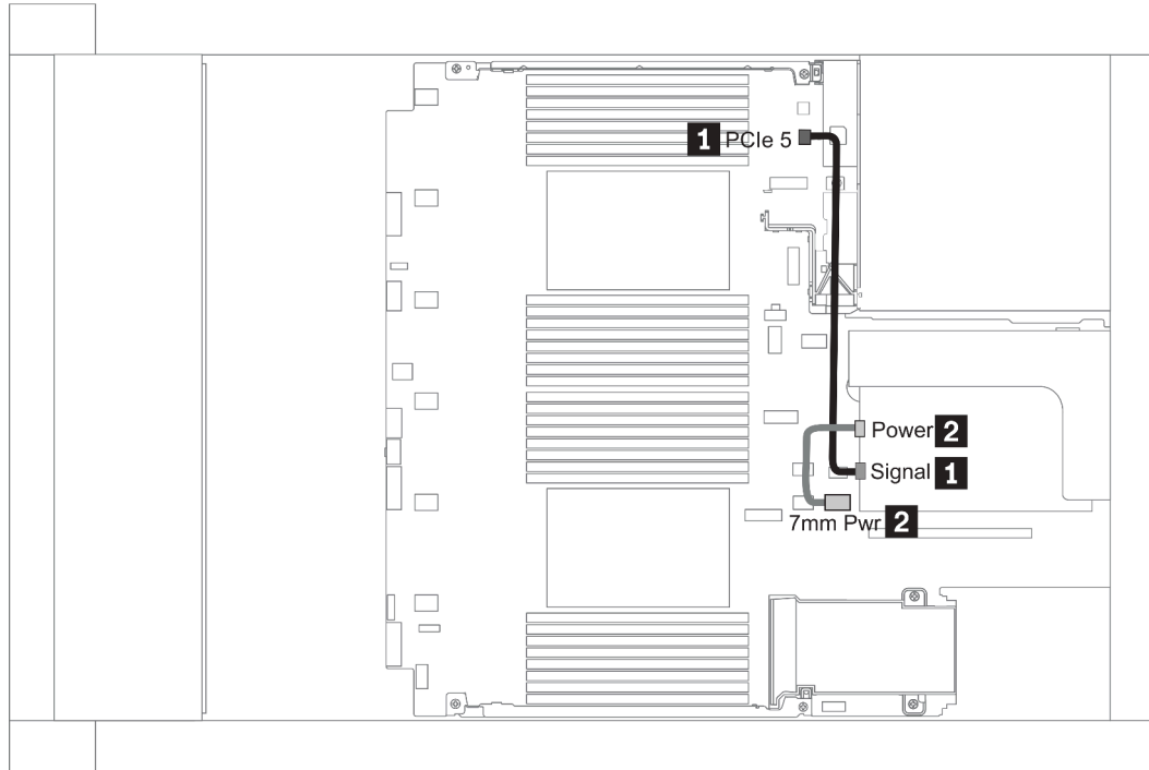
图 19. 7mm 线缆布放 when two processors installed
