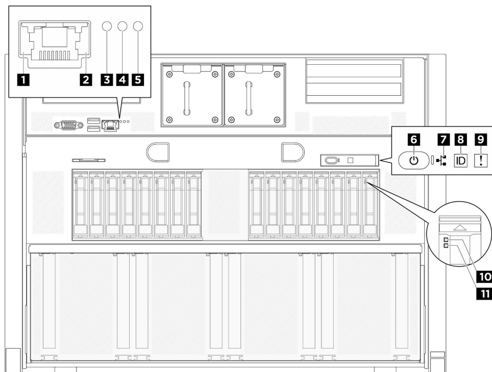
Figura 9. LED frontales
