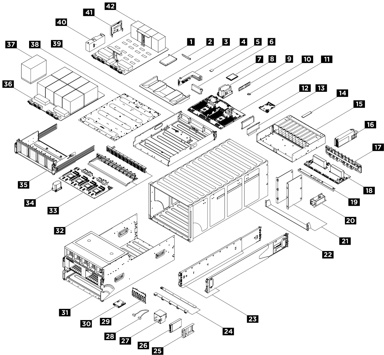
Figure 15. Composants serveur
