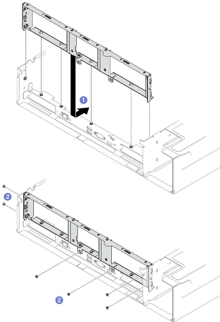
Figure 121. Installation du support mural arrière
