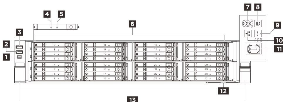
Figure 3. Front view of the sever model with E3.S 1T bays
