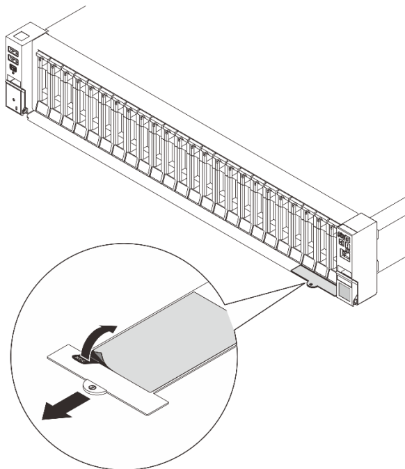
Figure 32. Lenovo XClarity Controller network access label on the pull-out information tab
