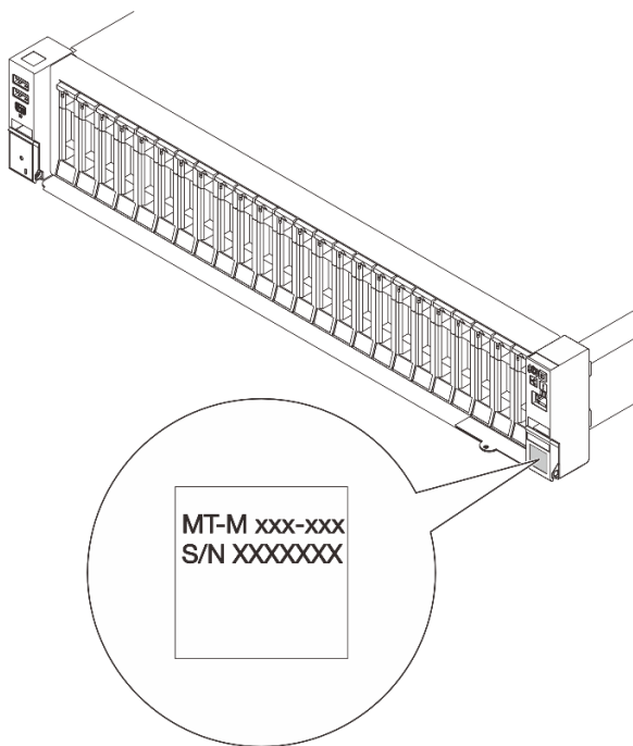
Figure 31. Location of the ID label
