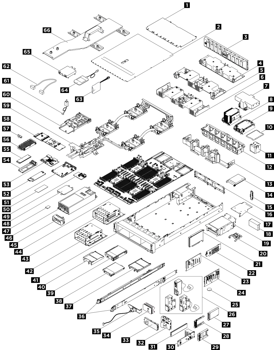
Figure 30. Server components
