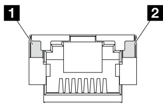
Figure 29. LEDs on the XCC system management port (10/100/1000 Mbps RJ-45)
