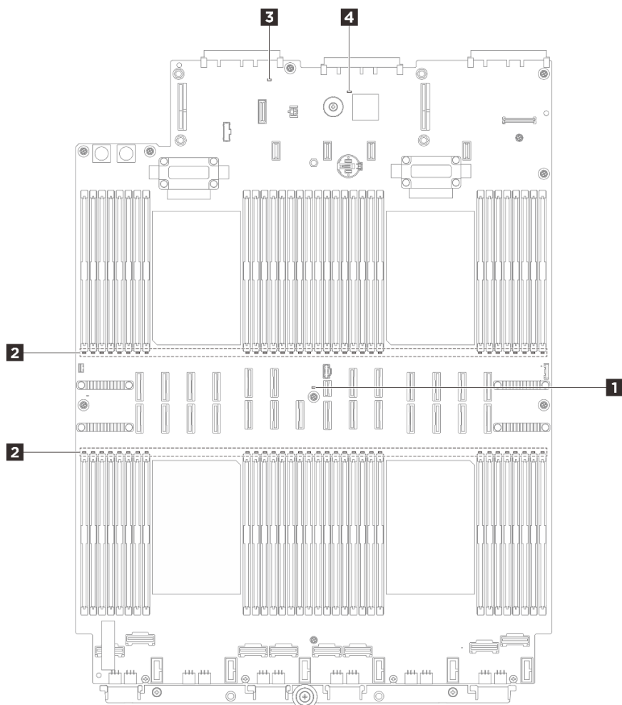
Figure 27. Processor board LEDs
