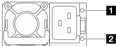
Figure 21. LEDs on a CRPS Premium (CFFv5) power supply unit
