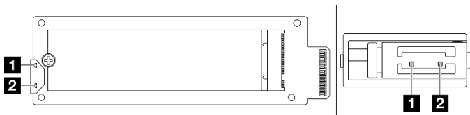
Figure 24. Rear M.2 interposer LEDs
