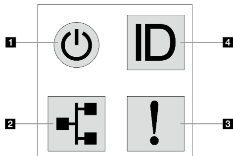
Figure 19. Diagnostics panel
