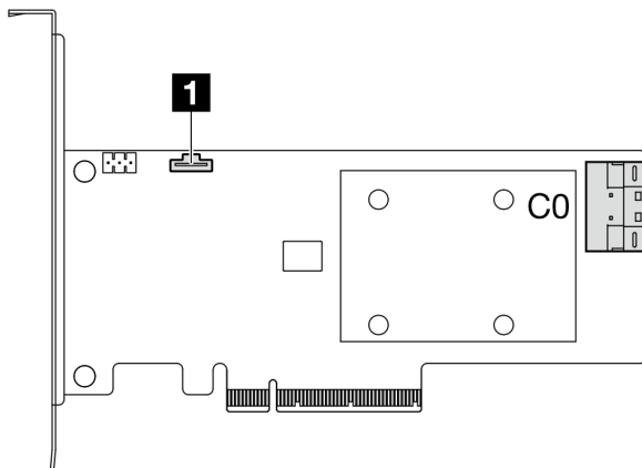
Figura 93. Conector 940-8i
