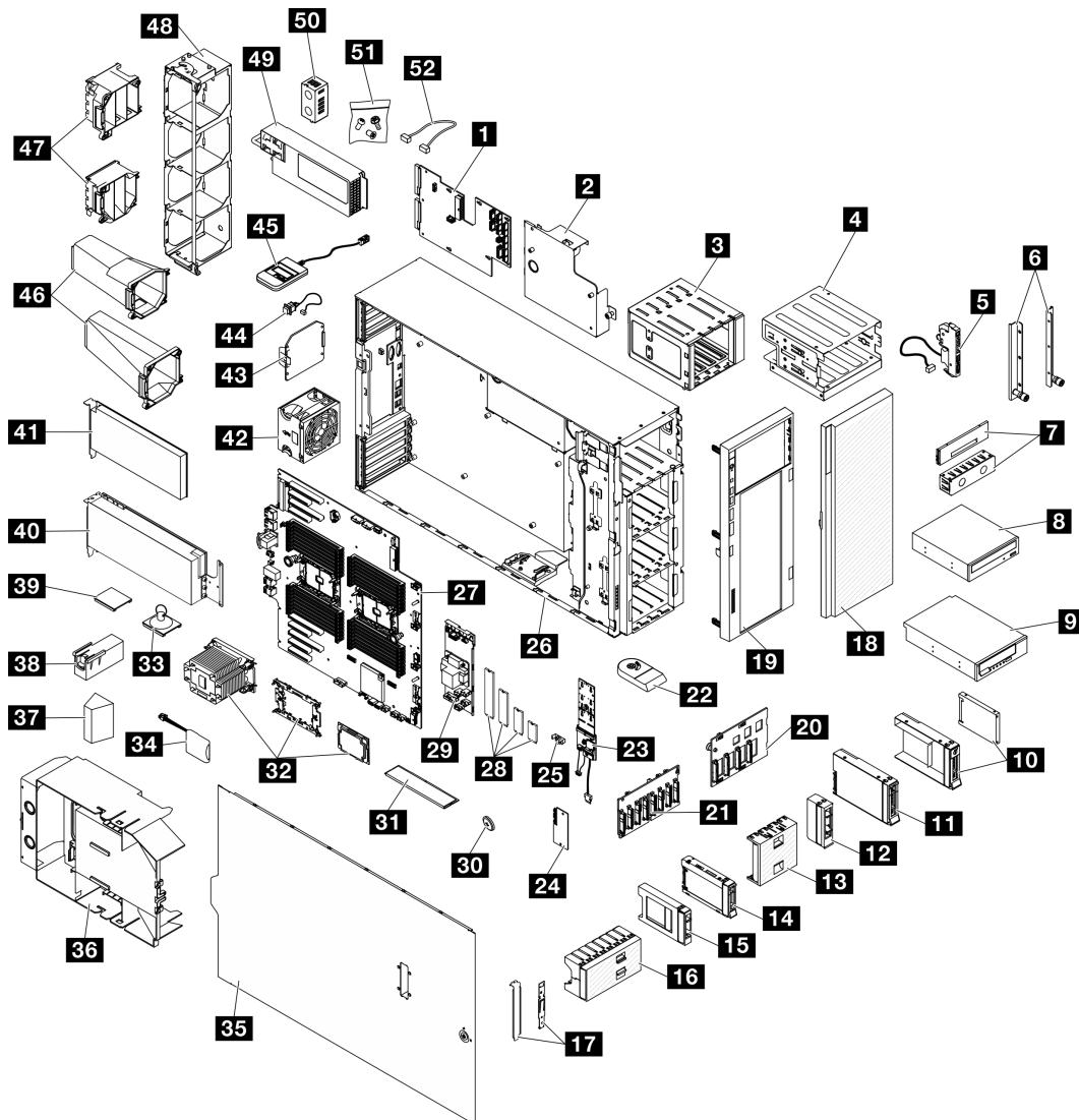
Figure 15. Composants serveur
